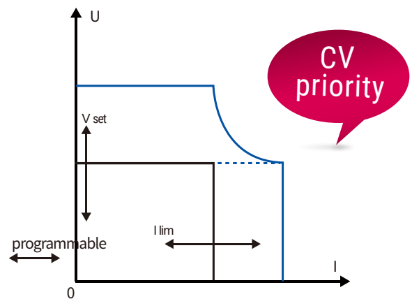
High-speed and seamless battery charging and discharging without overshoot (CV-High,CC-High,CCpriority)
