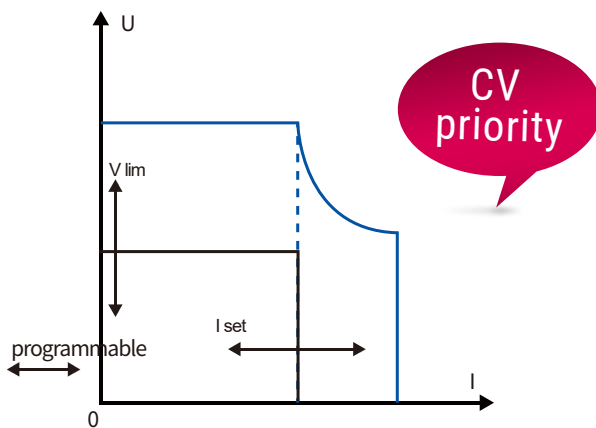
Starting surge current exceeds current range, high speed voltage (CV-High,CC-Low,CVpriority)
