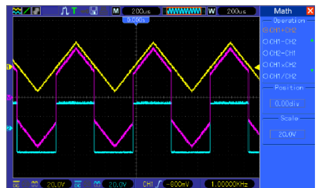
Math: CH1+CH2
